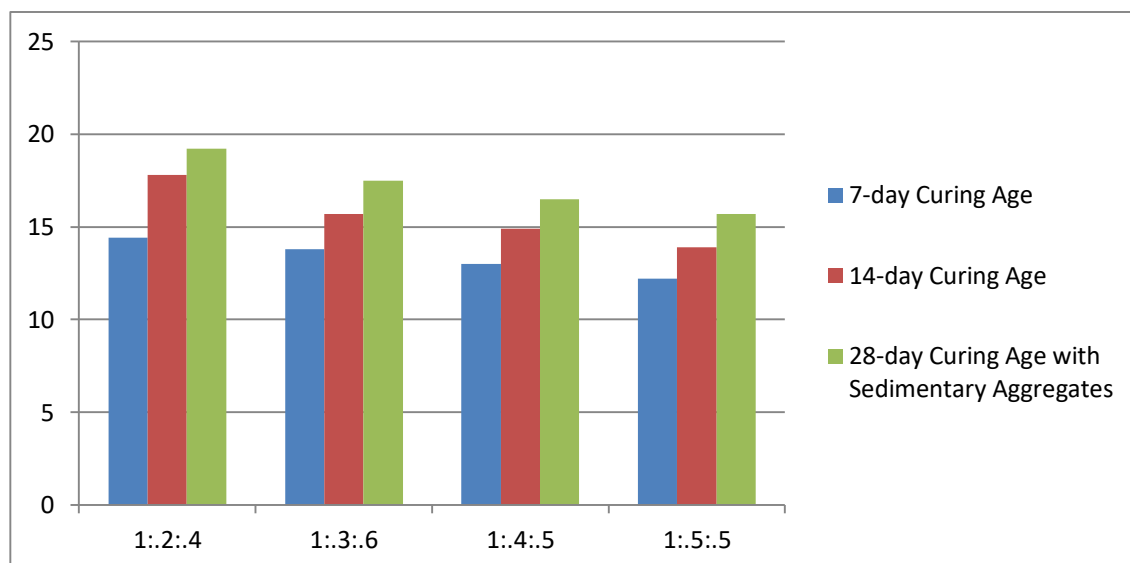
Fig 1. The Strength Values of the Respective Concrete Mixes with Sedimentary Aggregates through 7-day to 28-day Curing Ages
